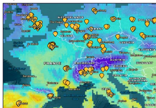
Map 22: Fire Weather Stress 2050, RCP 4.5
