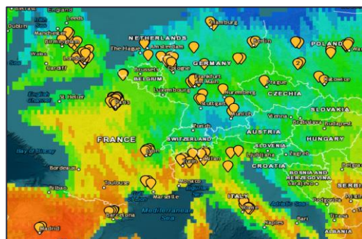
Map 11: Drought Stress 2030, RCP 8.5
