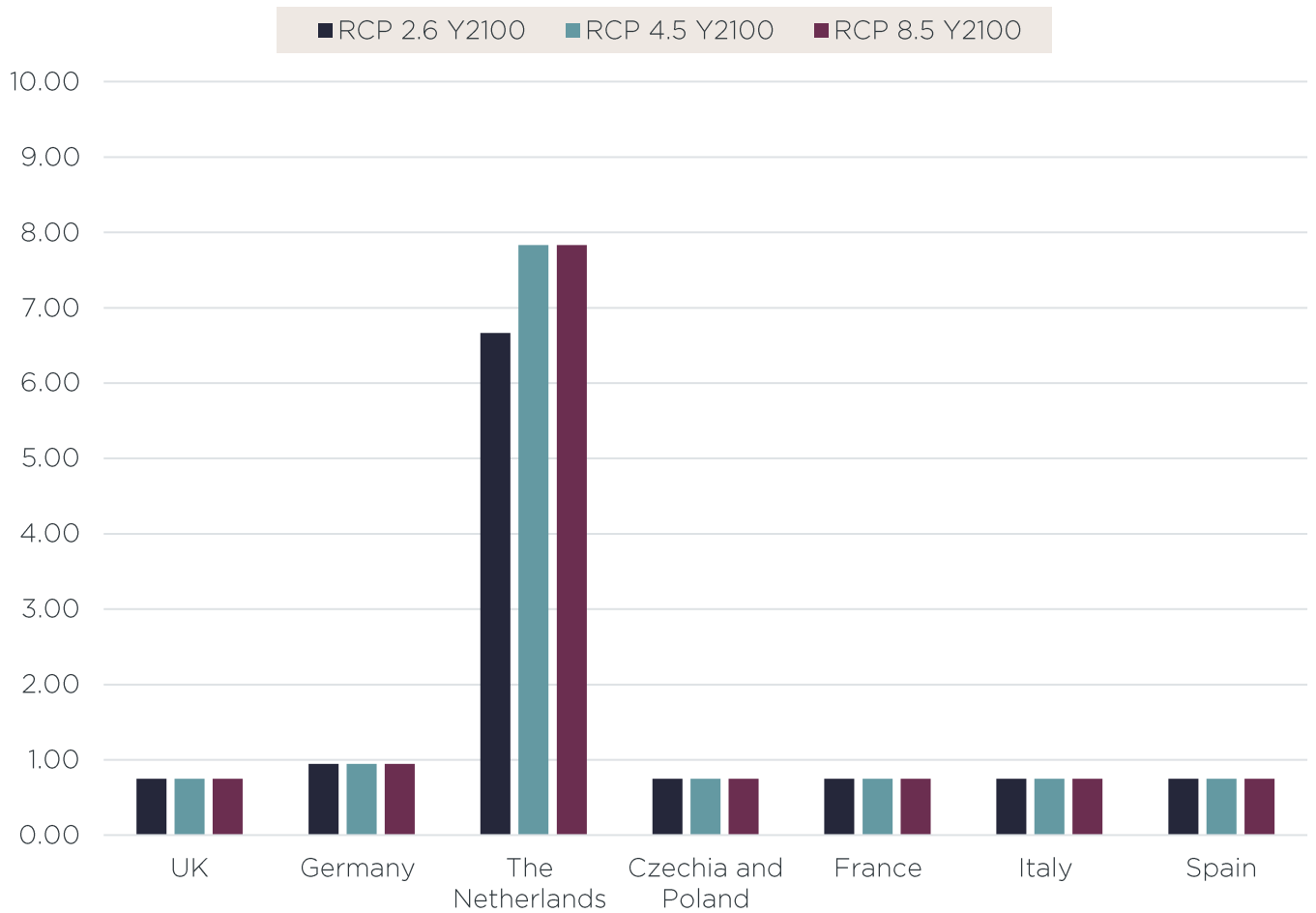
GRAPH 3: SEA LEVEL RISE. AVERAGE SCORE - ALL RCP AND TIME PERIODS, BY COUNTRY
