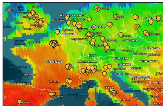
Map 12: Drought Stress 2050, RCP 8.5
