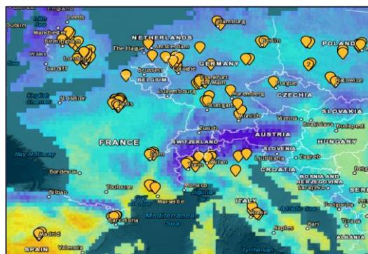
Map 21: Fire Weather Stress 2030, RCP 4.5
