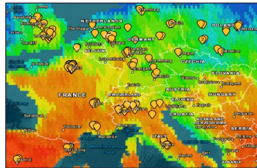
Map 10: Drought Stress 2050, RCP 4.5
