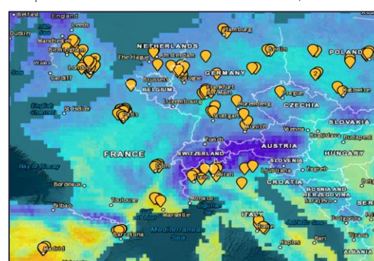
Map 23: Fire Weather Stress 2030, RCP 8.5
