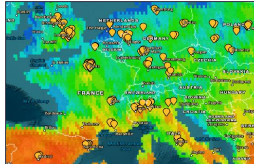
Map 9: Drought Stress 2030, RCP 4.5
