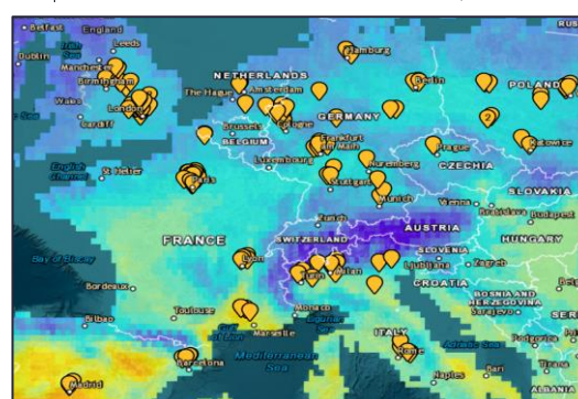
Map 24: Fire Weather Stress 2050, RCP 8.5
