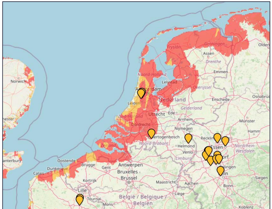
Map 2: Regional Sea Level Risk, RCP 8.5 2100
