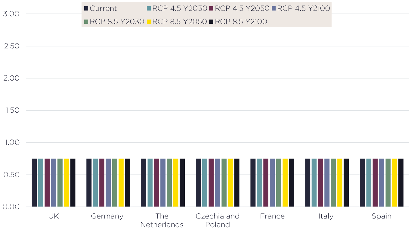
GRAPH 5: TROPICAL CYCLONE. AVERAGE SCORE - ALL RCP AND TIME PERIODS, BY COUNTRY
