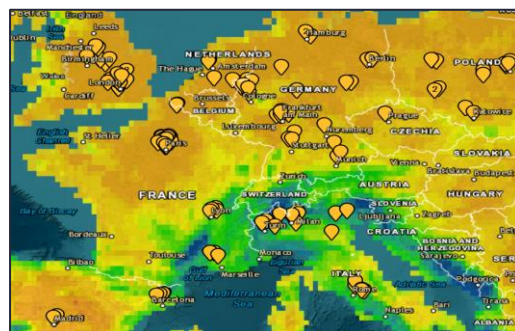
Map 13: Precipitation Stress 2030, RCP 4.5
