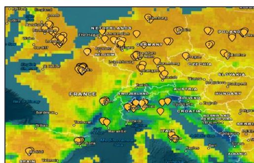
Map 15: Precipitation Stress 2030, RCP 8.5
