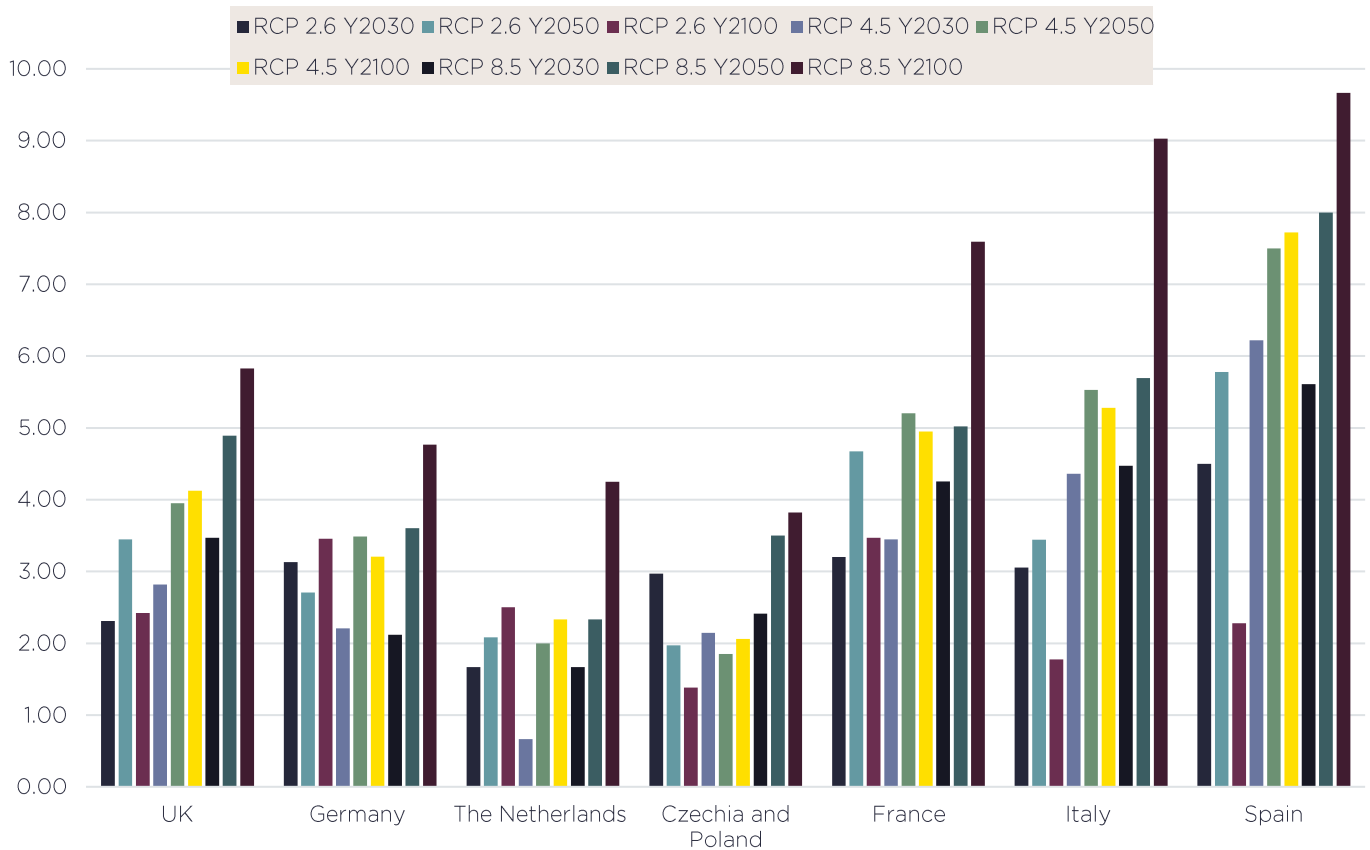
GRAPH 6: DROUGHT STRESS. AVERAGE SCORE - ALL RCP AND TIME PERIODS, BY COUNTRY
