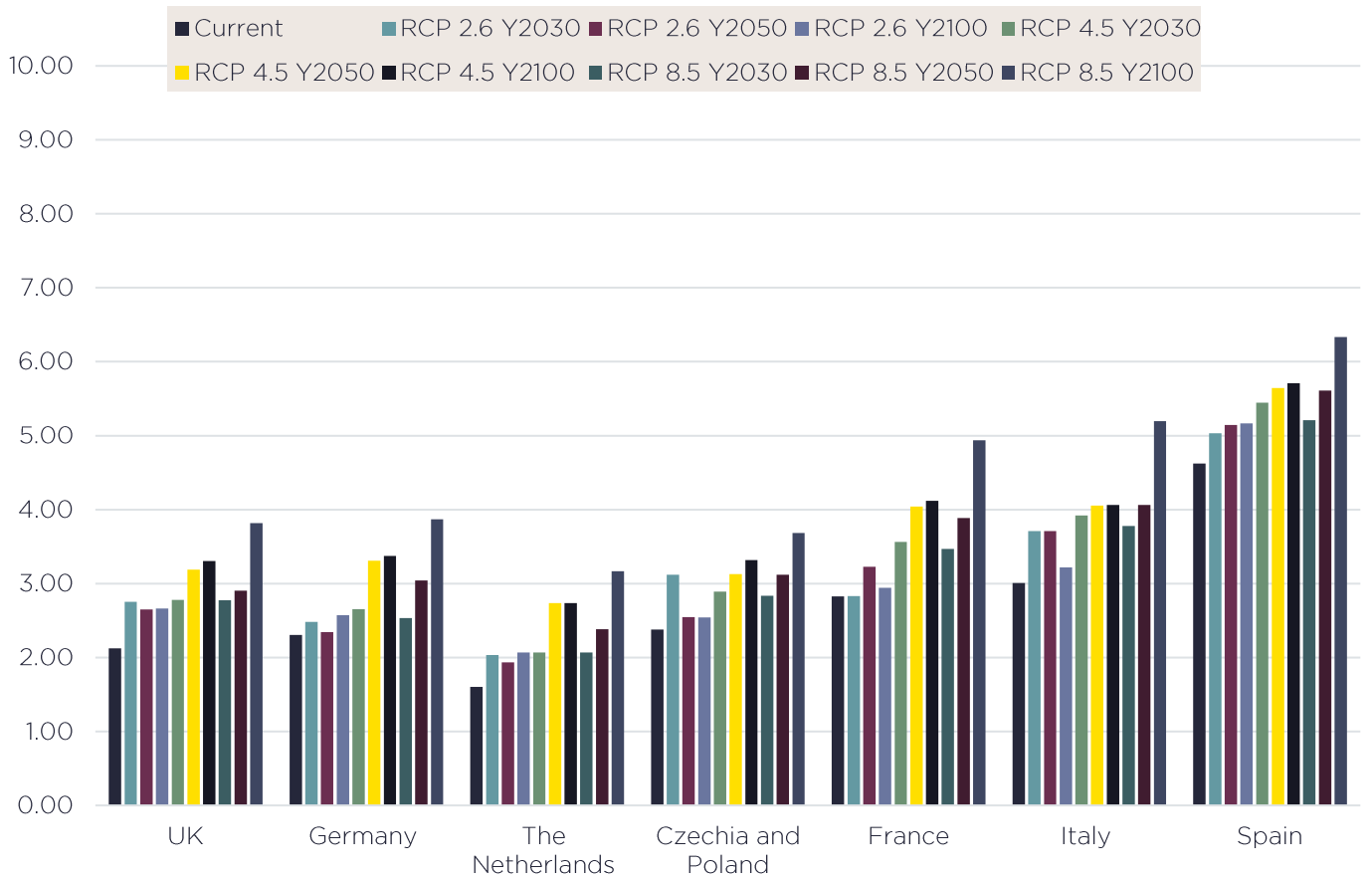
GRAPH 9: FIRE WEATHER STRESS. ALL RCP AND TIME PERIODS, BY COUNTRY
